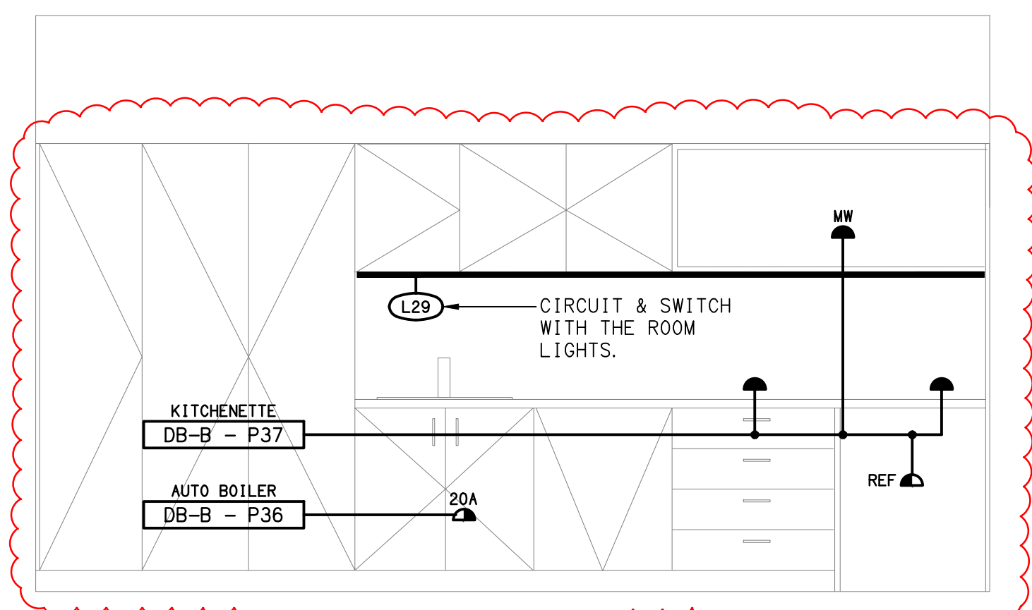
DETAIL A WORK AREA KITCHENETTE ELEVATION SCALE 1:25
